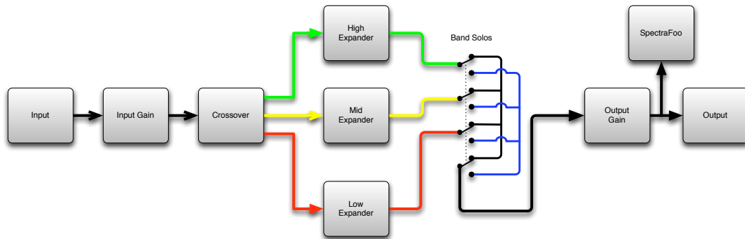
Figure 5.1: Multiband Expander Signal Flow
