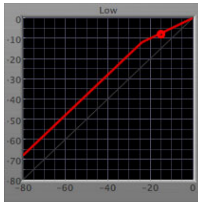
Figure 4.14: Dynamics Knee
